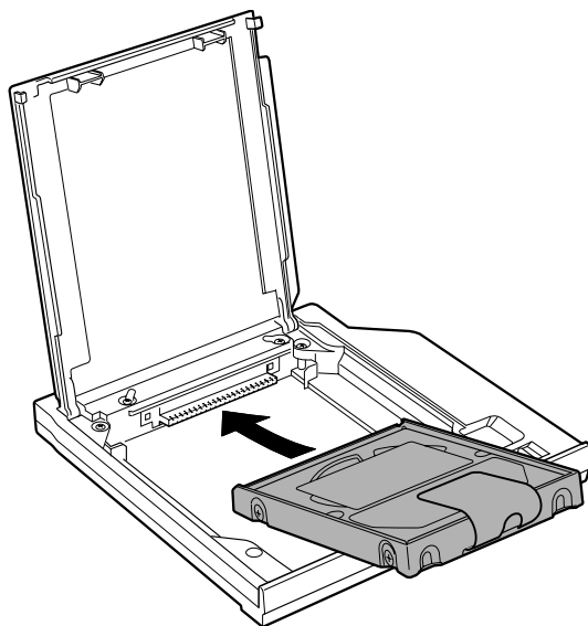
Installing the HDD
