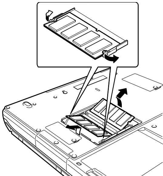
Opening the lid
