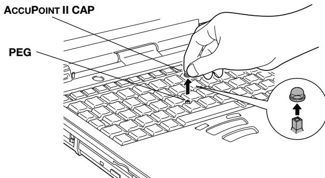
Removing the AccuPoint II cap
