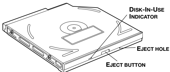
The optical media device
