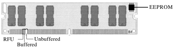
Figure 2-5: 168-pin DIMM
