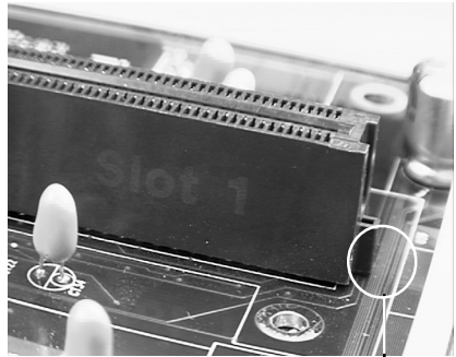
Figure 2-8 - Pentium II Slot Connector and Key Pin
