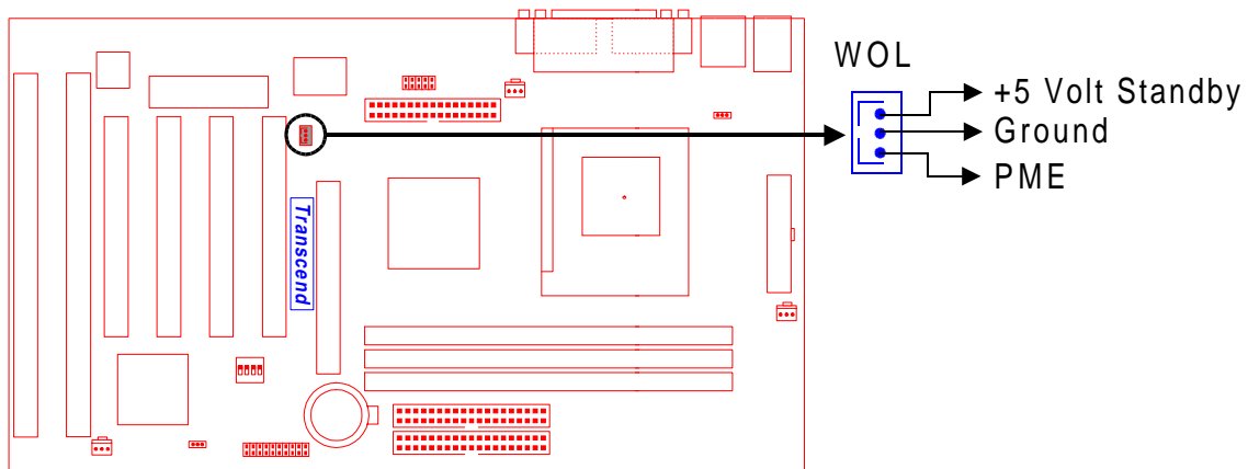
TS-ABX31 Wake-on-LAN Connector
