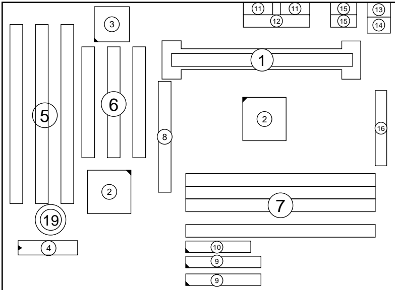
Figure 1-1. Mainboard Layout
