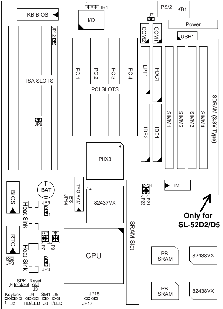
Figure 1-1. SL-52D2/D5/E2/E5 Motherboard Layout
