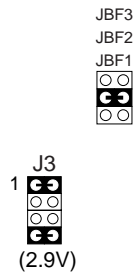
Figure 2-2. CPU Type Configuration
