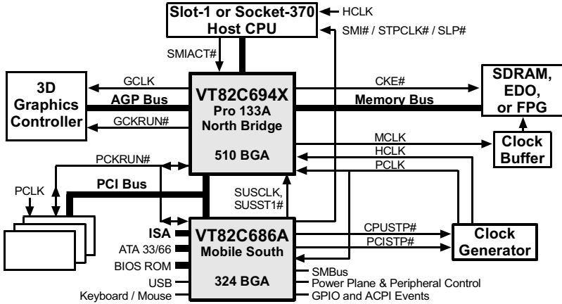
Apollo Pro 133A system with VT82C686A Mobile South-Bridge.
