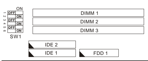
Figure 2-1. CPU Type Configuration
