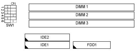
Figure 2-3. CPU Type Configuration
