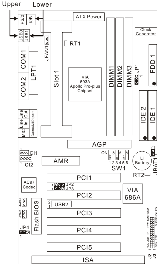
Figure 1-1. Motherboard Layout
