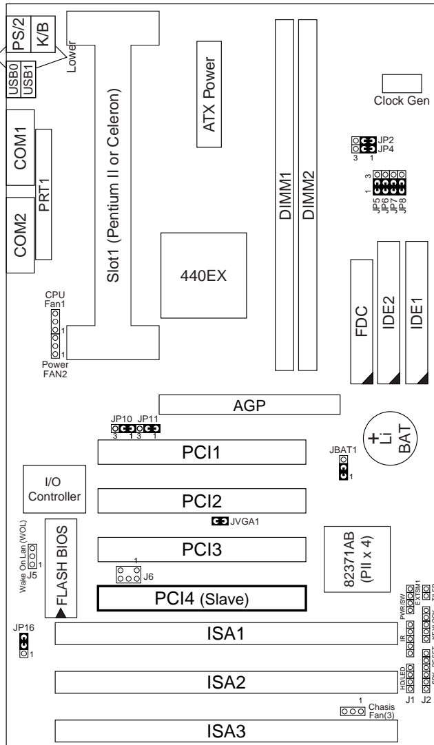
Figure 1-1. Motherboard Layout
