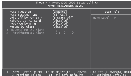
Power Management Setup 设置菜单
