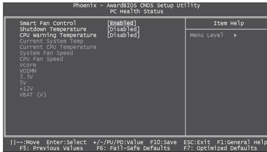
PC Health Status 菜单
