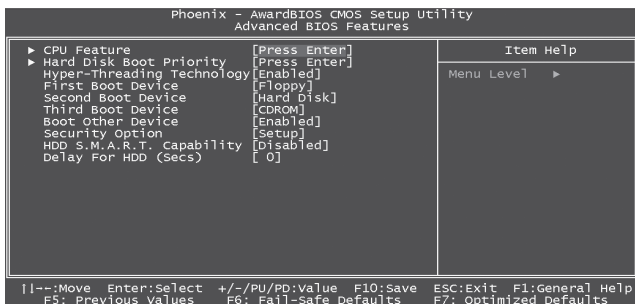
Advanced BIOS Features 设置菜单
