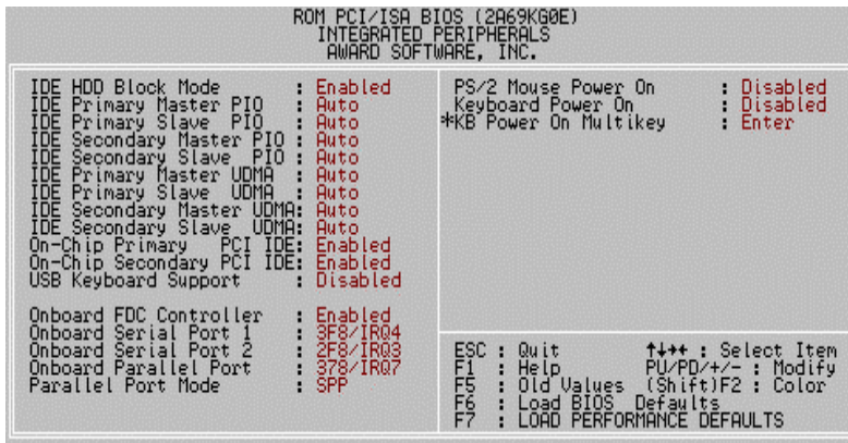
Figure 4.9: Integrated Peripherals
