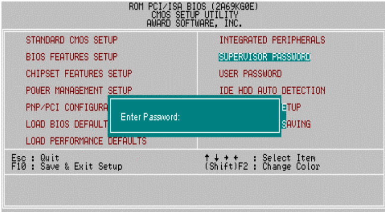
Figure 4.10: Password Setting
