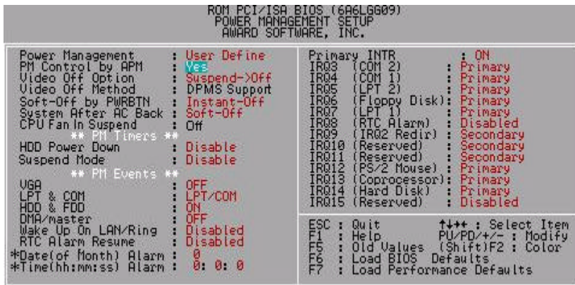
Figure 4.5: Power Management Setup
