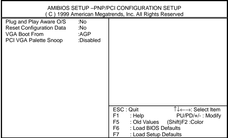
Figure 6: PnP/PCI Configuration
