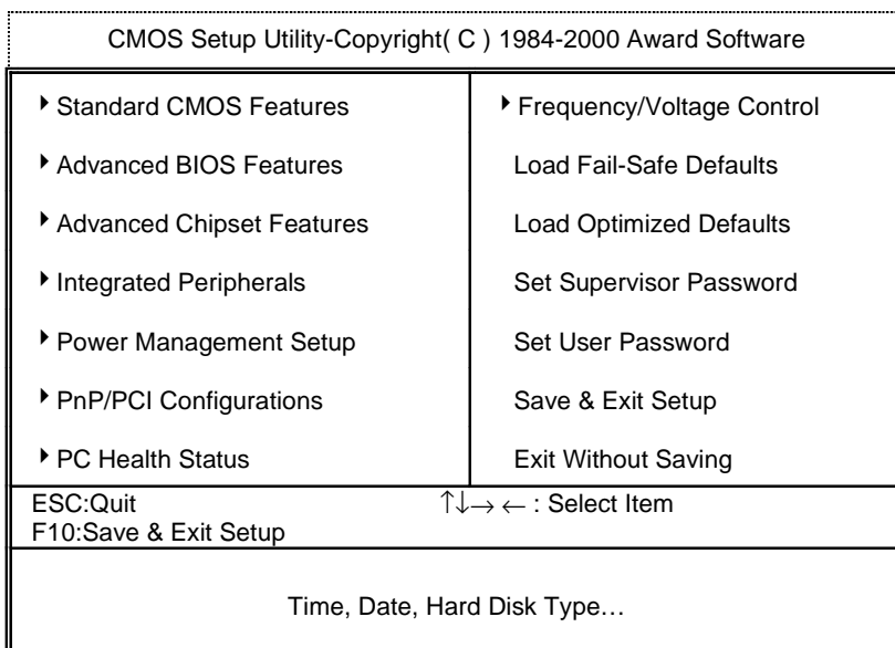
Figure 2: Main Menu
