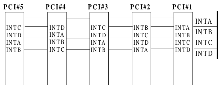
Figure 3-7: The Combination of PCI INT#lines
