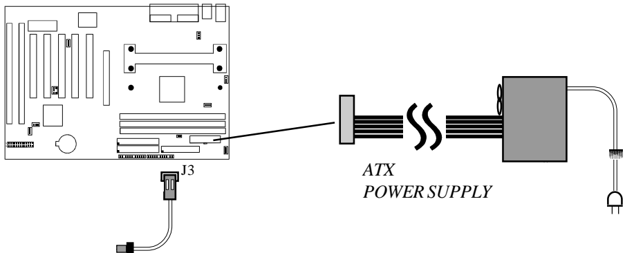
P2-133A Board Case (chassis) Power ON/OFF button
