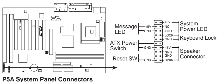
P5A System Panel Connectors
