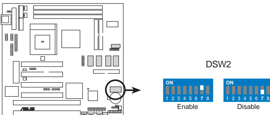
ME-99B LCD Setting
