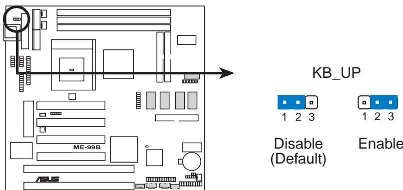
ME-99B Keyboard Power Up
