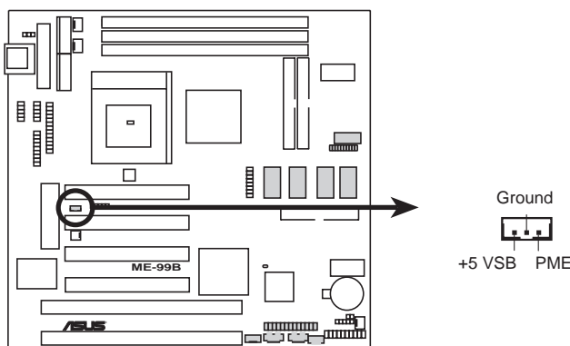
ME-99B Wake-On-LAN Connector
