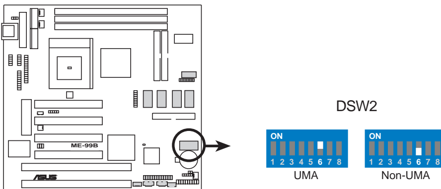
ME-99B Display Memory Setting
