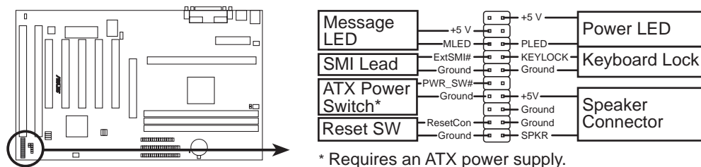
P2L97 System Panel Connections
