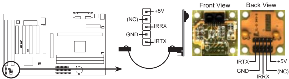
Infrared Module Connector
