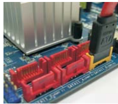
Connect the SATA data cable to the orange SATAII connector (SATAII_6 (PORT5))
