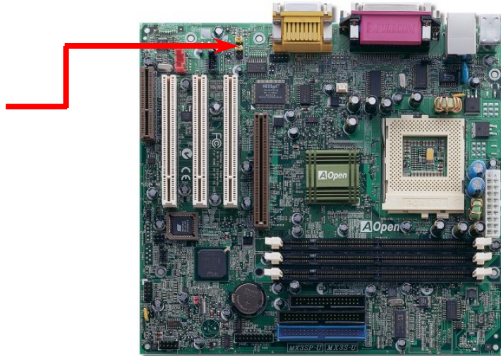
Front Audio Connector
