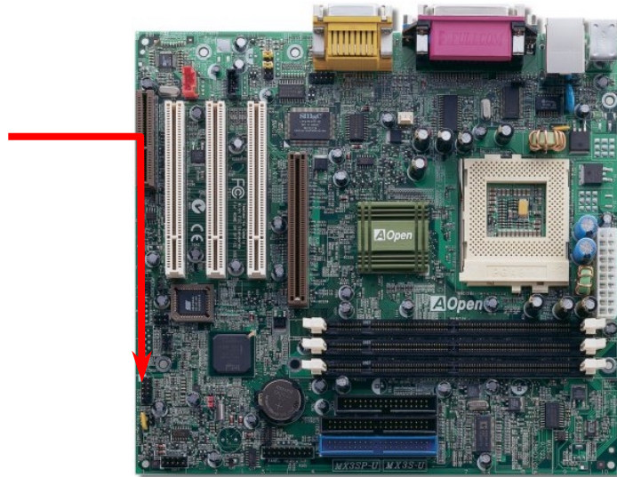
USB2 Connector
