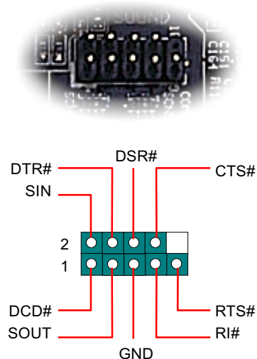
COM2 Conector
