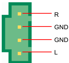
VIDEO-AUDIO-IN
