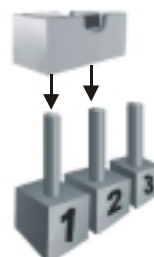
Pin1-2 close
