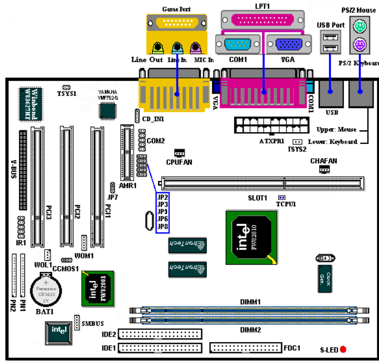
Figure 1-3. Motherboard component location
