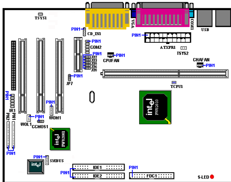
Figure 2-7. All Connectors and Headers for the WB6
