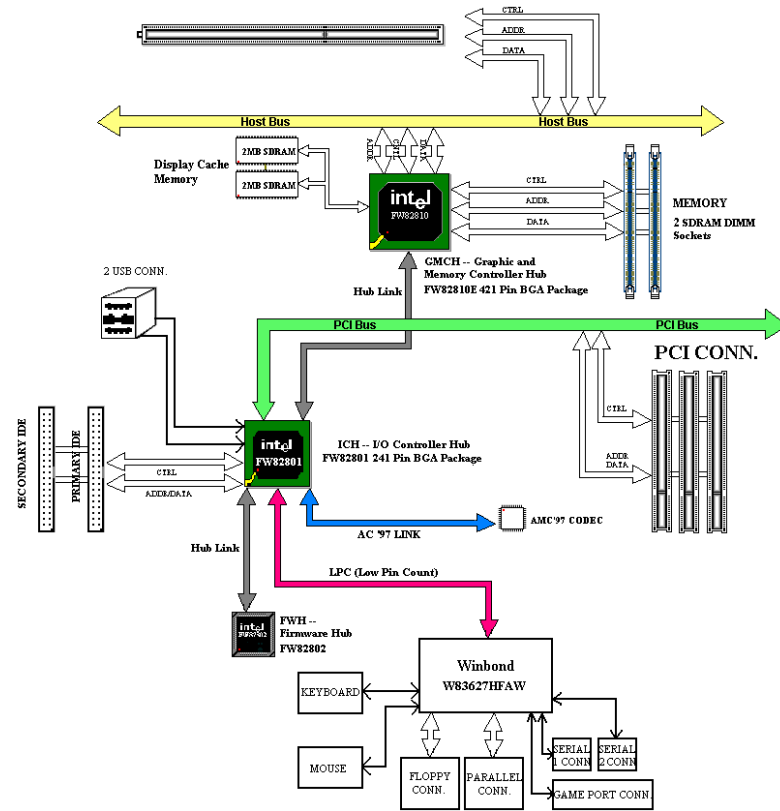
Figure 1-4. System diagram of the WB6 mainboard
