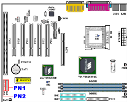
Figure 2-9. The definition of PN1 and PN2 pins
