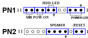
Figure 2-9. The definition of PN1 and PN2 pins
