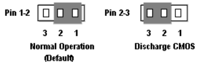
Figure 2-8. CCMOS1 jumper setting
