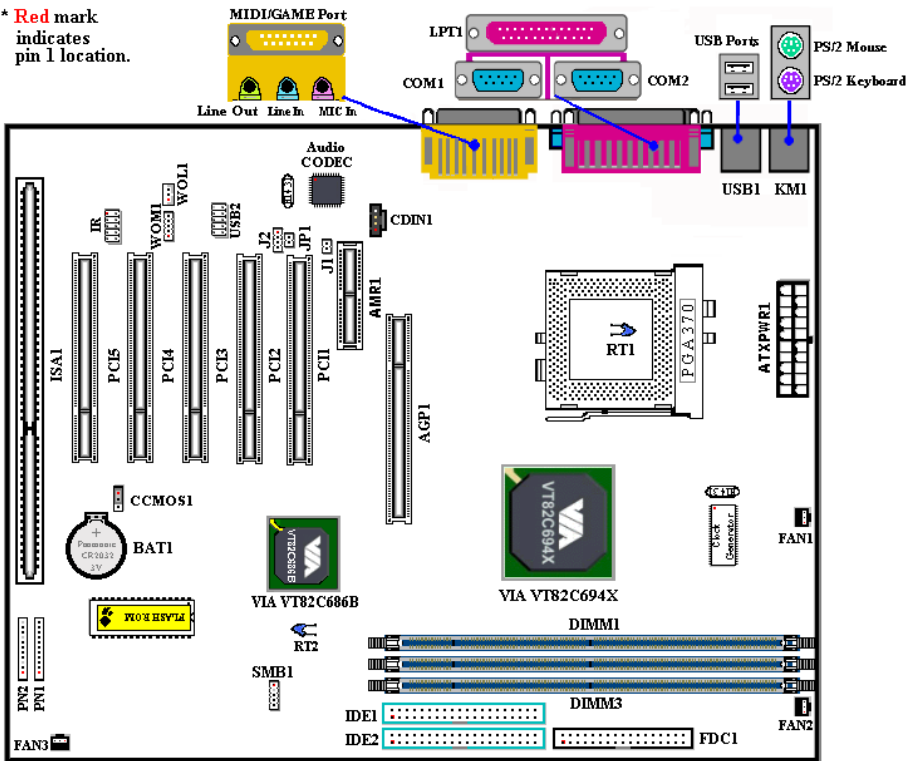
Figure 1-1. VH6/VH6-II/VH6T Motherboard component location (Note that the components placement of BAT1 and CCMOS1 is slightly different between these three models.)
