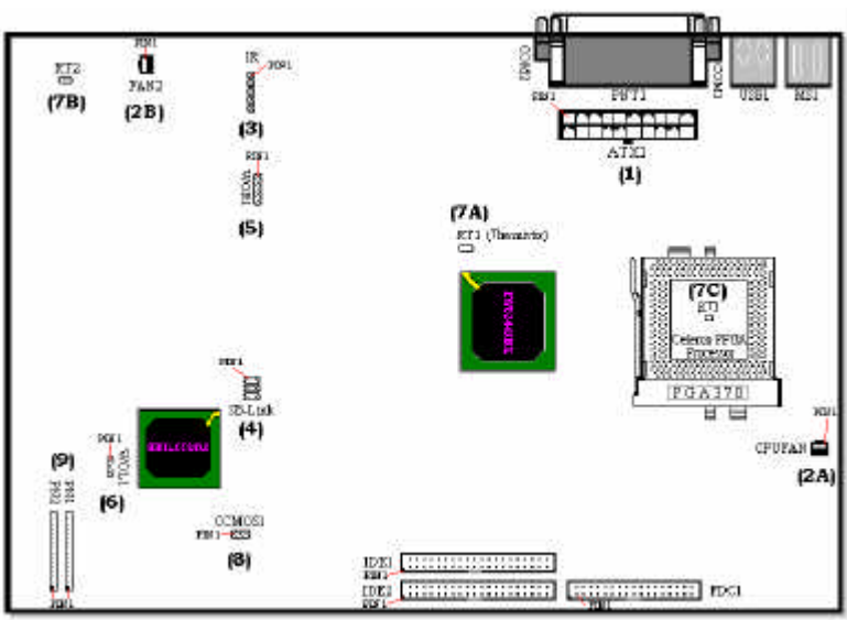
Figure 2-7. All Connectors and Headers for the BM6
