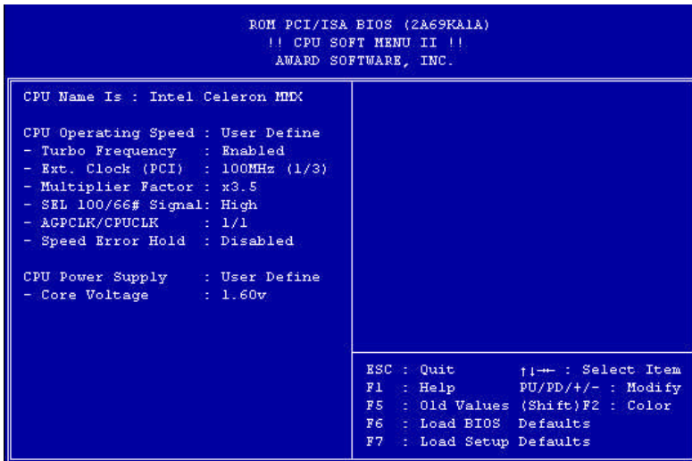
Figure 3-2. CPU SOFT MENU™ II
