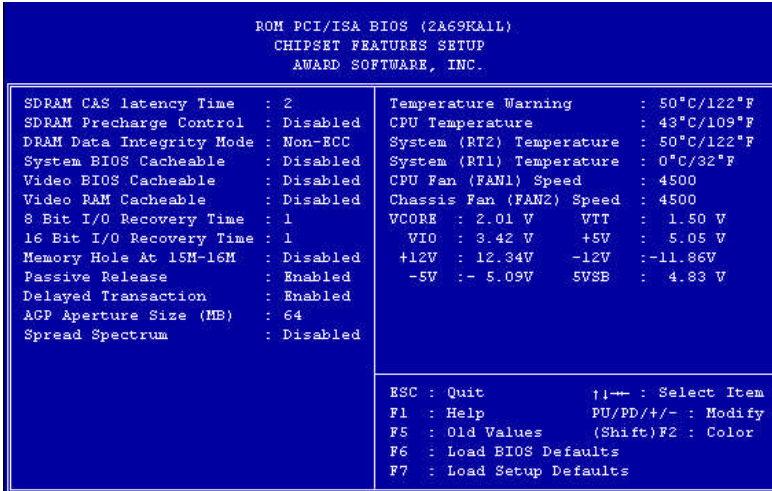
Figure 3-5. Chipset Features Setup
