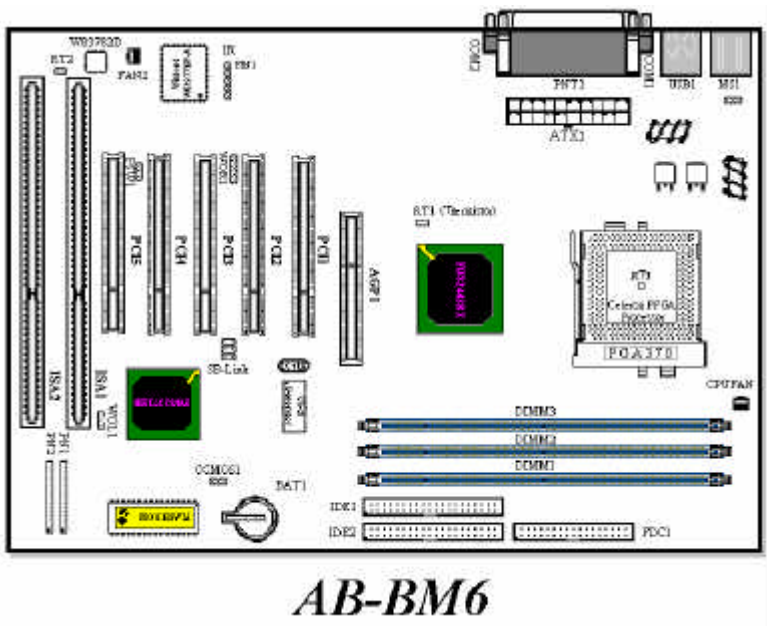
Figure 1-2. Motherboard component location
