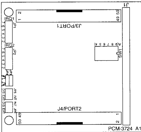
Jumper and switch locations
