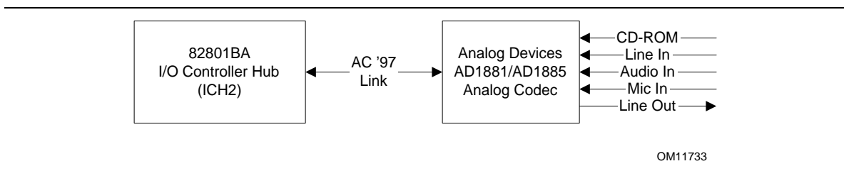
Figure 4. Audio Subsystem Block Diagram
