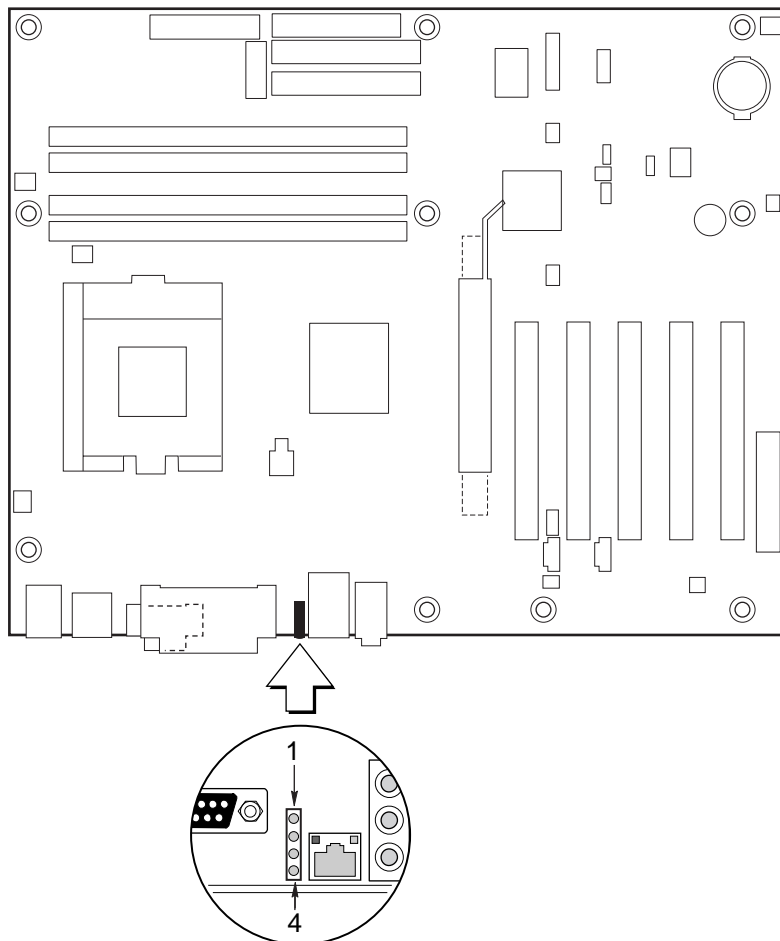
Figure 17. Diagnostic LEDs
