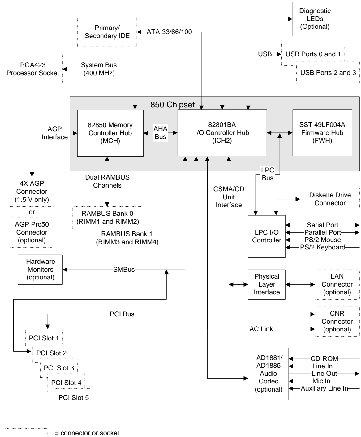
Figure 2. Block Diagram
