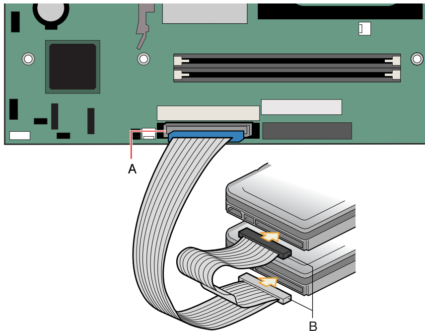
Figure 9. Connecting the IDE Cable
