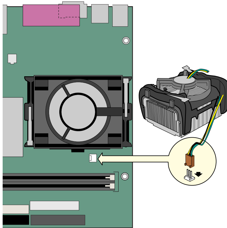
Figure 6. Connecting the Processor Fan Heat Sink Cable to the Processor Fan Connector
