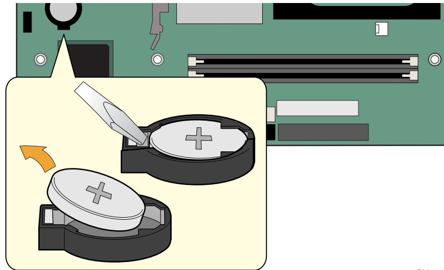
Figure 15. Removing the Battery
