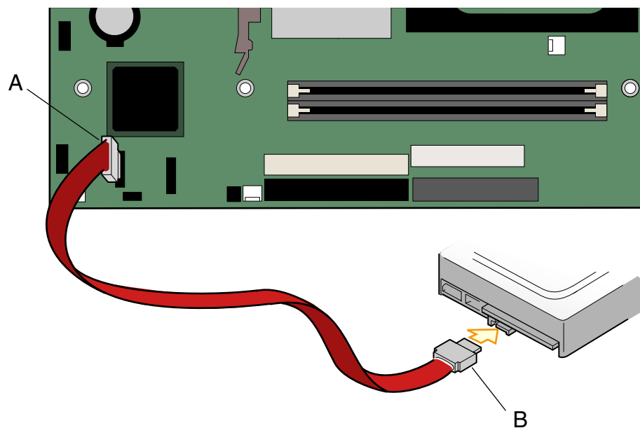
Figure 10. Connecting the Serial ATA Cable
