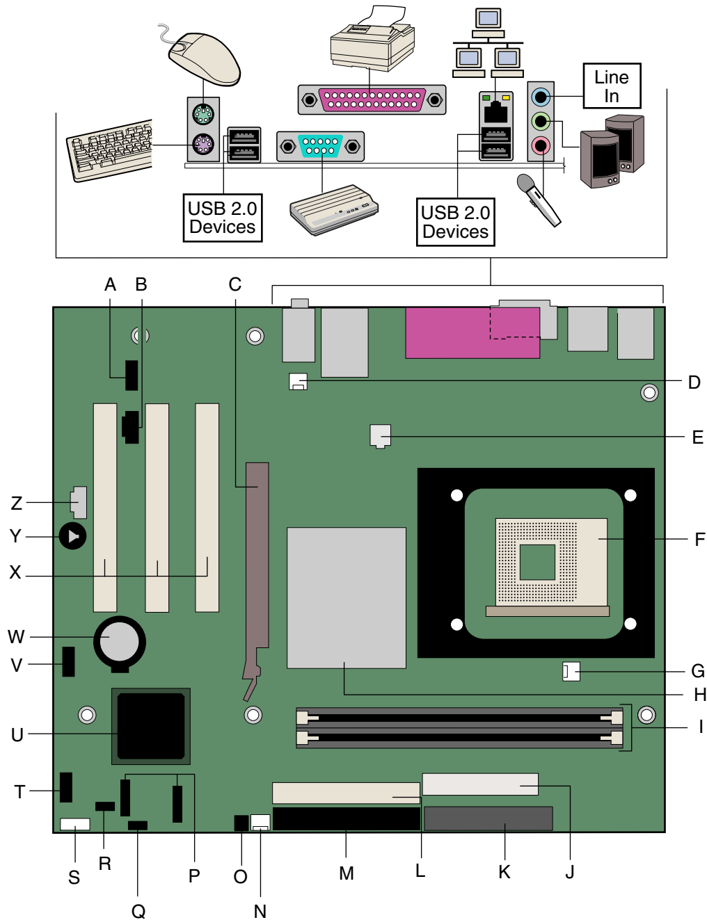
Figure 1. Desktop Board Components
