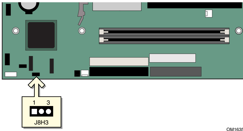
Figure 14. Location of the BIOS Configuration Jumper Block
