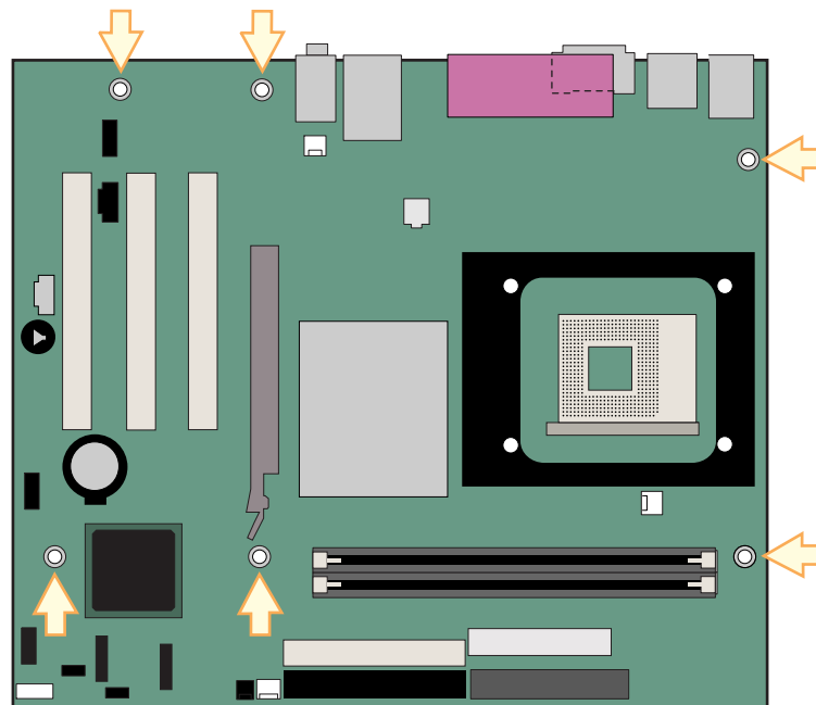
Figure 4. Location of Desktop Board Mounting Screw Holes
