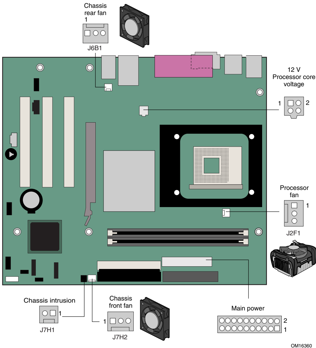
Figure 13. Location of Hardware Control Headers and Power Connectors
