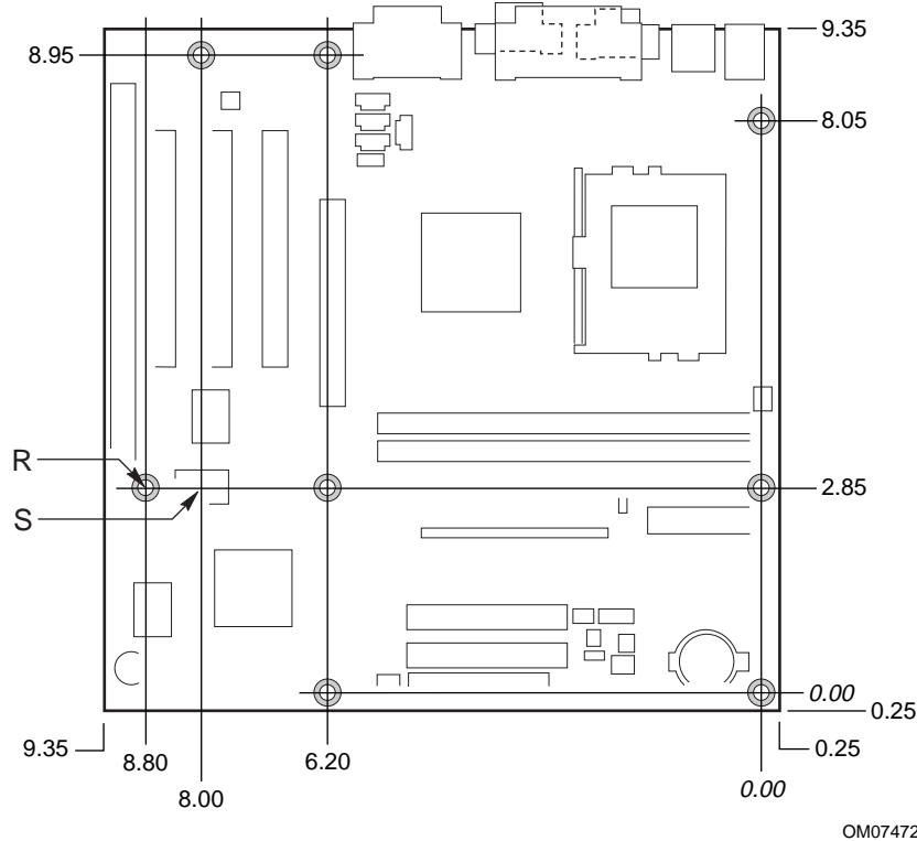
Figure 10. Motherboard Dimensions
