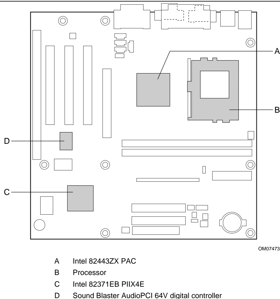
Figure 13. Thermally-sensitive Components
