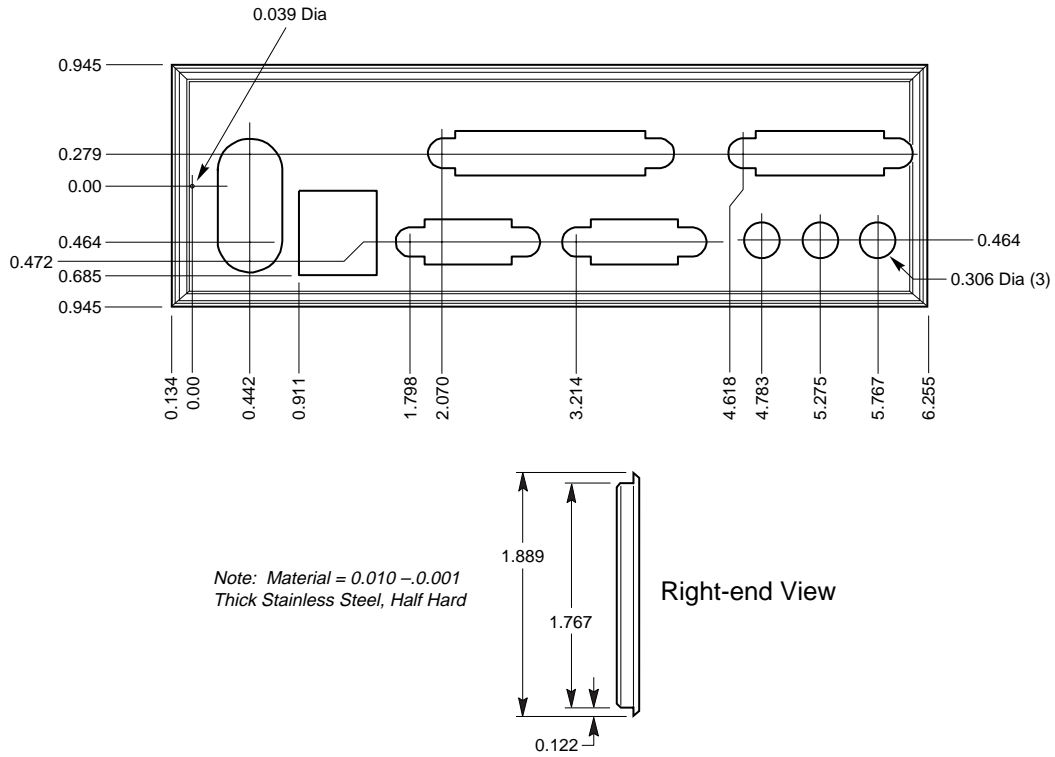
Figure 12. Back Panel I/O Shield Dimensions (ATX/microATX Chassis-Independent)
