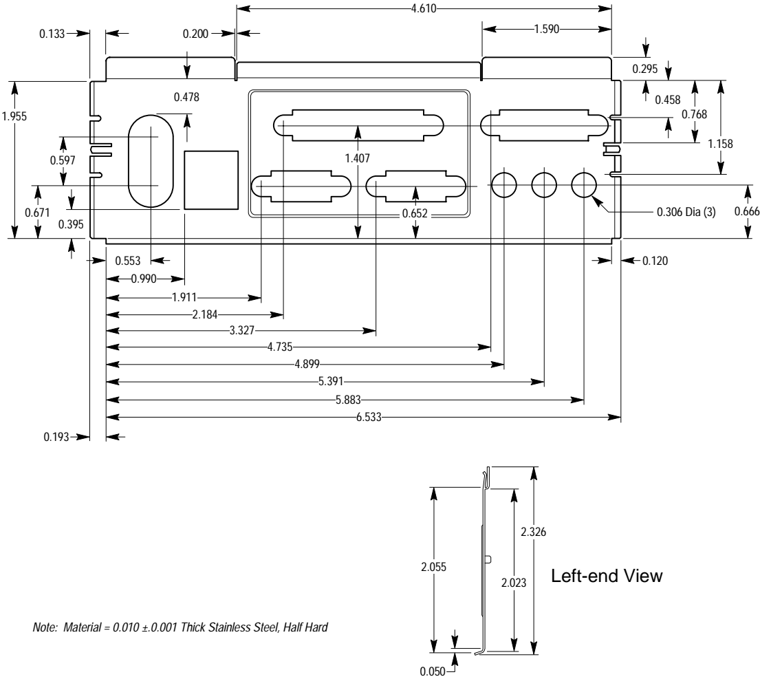
Figure 11. Back Panel I/O Shield Dimensions (Intel® ATX/microATX Chassis)
