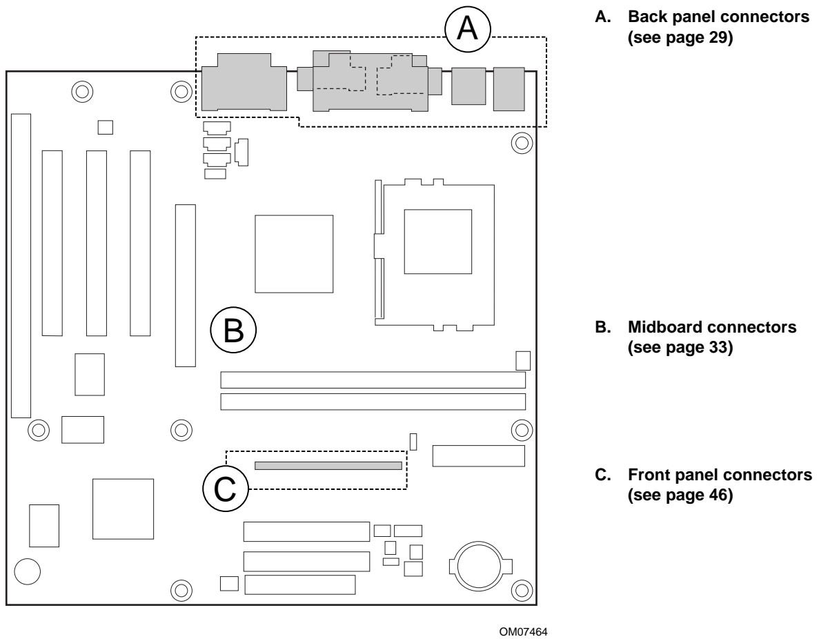
Figure 2. Connector Groups
