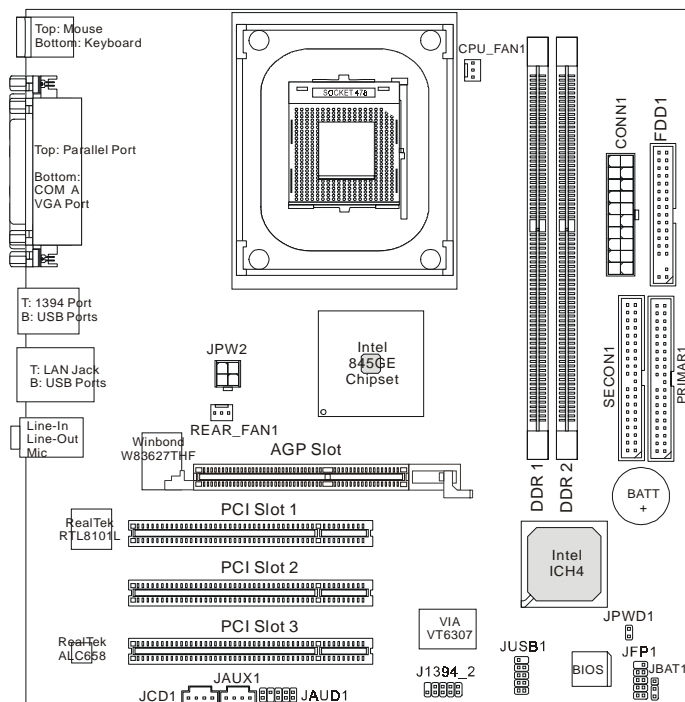
MS-6577 v4.X Micro ATX Mainboard
