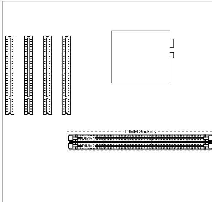
Figure 4-3. DIMM Module Locations
