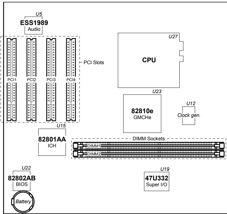
Figure 2-1. Major Components of System Board
