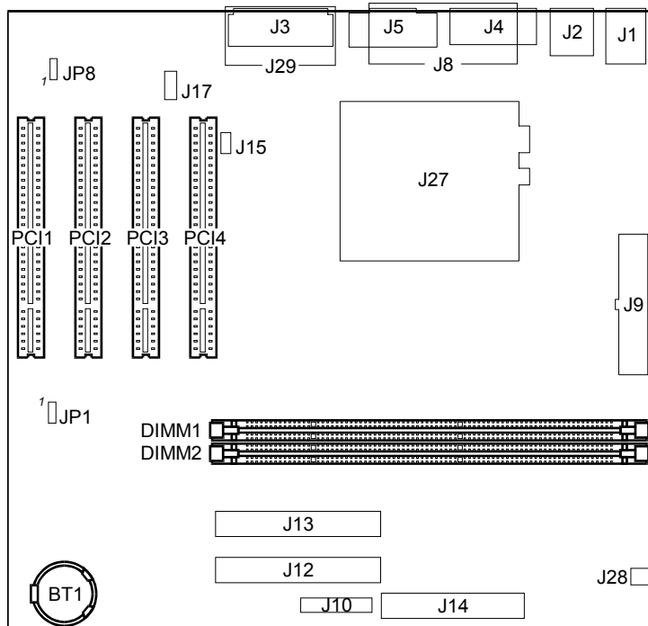
Figure 3-1. Connector and Jumper Locations
